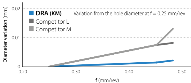
Hole diameter variation related to feed rate (Internal evaluation)
